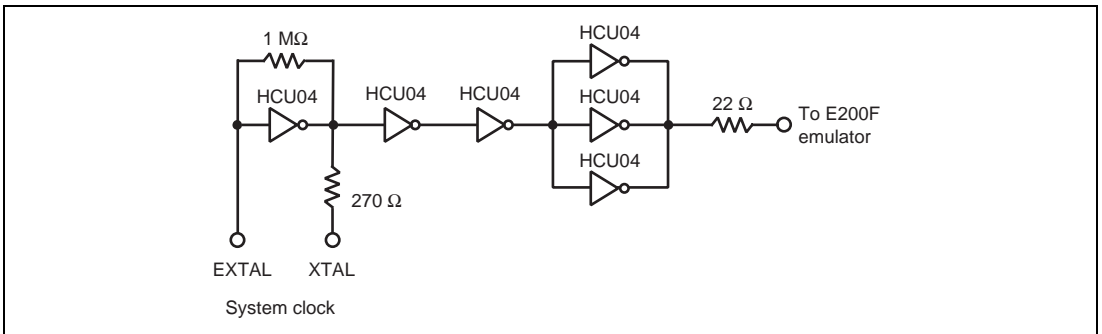
Figure 8 Clock Oscillator
